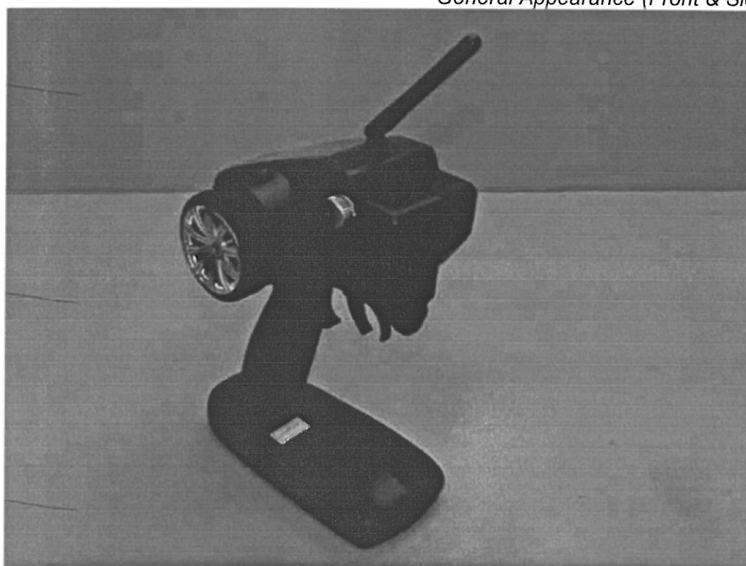
Figure 2 General Appearance (Front & Side View)
